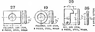
Figs. 1373-1376. Side-stem Follower.
